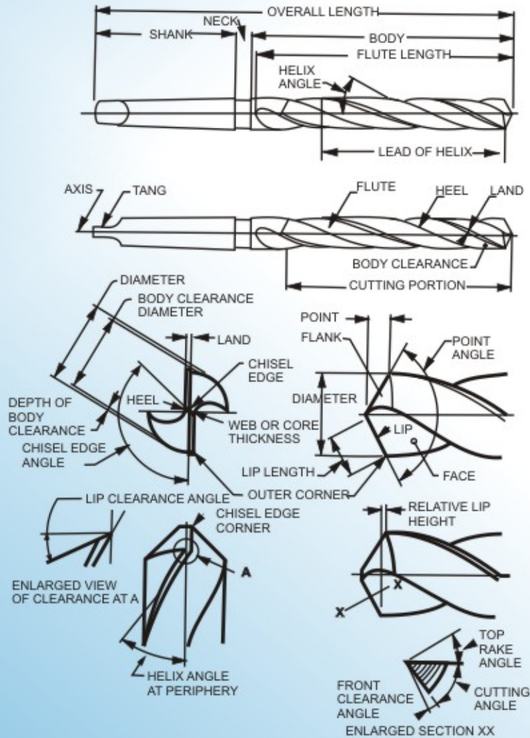
Twist drill with Taper shank
